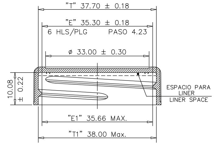
SECCION "B-B" SECTION "B-B"
